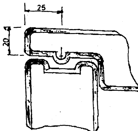
Fig. relation of the box & lid. SHAPE OF THE UNDERSIDE OF THE LID
